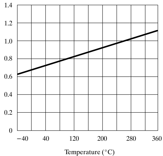
Figure 5b. Specific Heat of Silicon vs. Temperature ( W \text{ sec}/gm^{\circ} )
