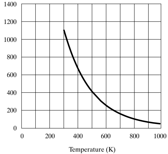
Figure 5a. Conductivity of Silicon vs. Temperature ([Physics Review, Vol. 130 (6/'63)] ( W/cm^{\circ} )
