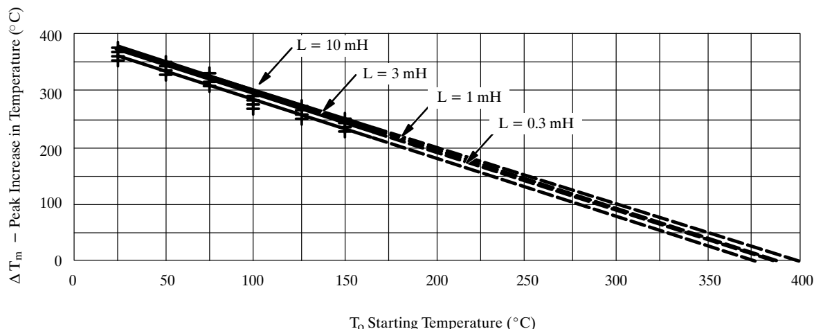
Figure 10. Temperature Increase vs. Starting Temperatures
